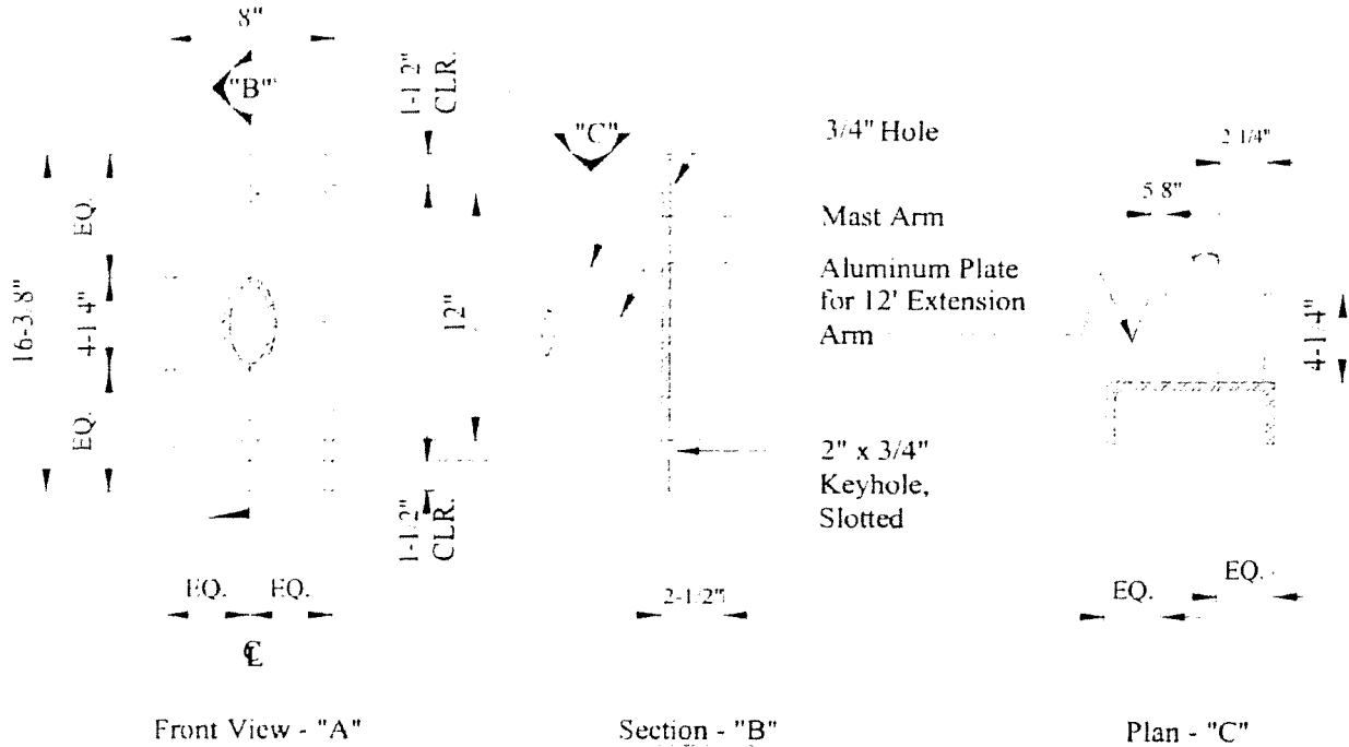
Mounting Plate Detail Figure 2
